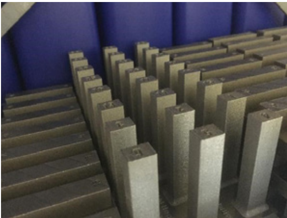
AM Dievar vs 1.2709 and AM H13, printed vertical direction and heat treated to hardness range of 46-48 HRC. The fine grain structure of AM Dievar results in superior high toughness values.
