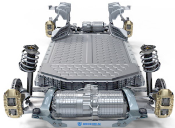
E-mobility – picture showing e.g. battery box, electrical motor housing and structural parts on an EV car.
