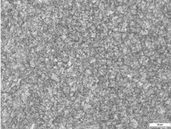
Microstructure in hardened tempered condition, magnification 500x.
